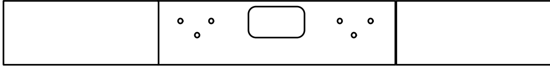
FREIGHTLINER CORONADO 12" HD, 3" TOP LIP, SET-BACK, 3/8" STEEL 2010 - current
