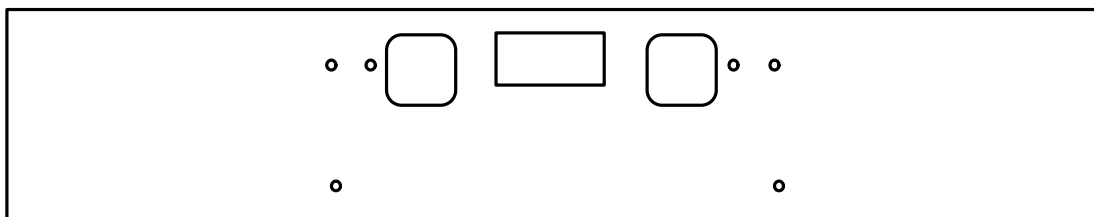
18" TEXAS STYLE WITH ROLLED ENDS, 3/16" STEEL
